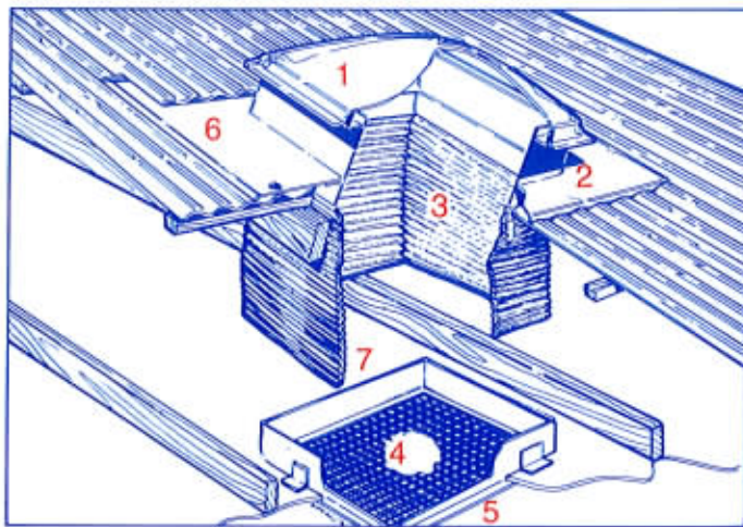
Diagram 1 Showing ventilated area and air-flow movement.
