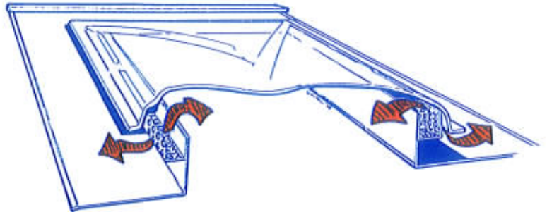
Diagram 1 Showing ventilated area and air-flow movement.
